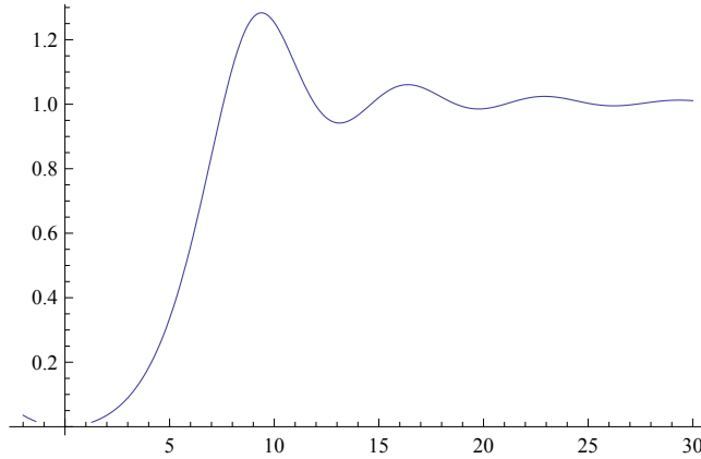
Figure 1.2: The normalized pair correlation function k^\theta(\lambda) in the \frac{\partial}{\partial\theta} tangent direction u^\theta for the sphere in \mathbb{C}^2
