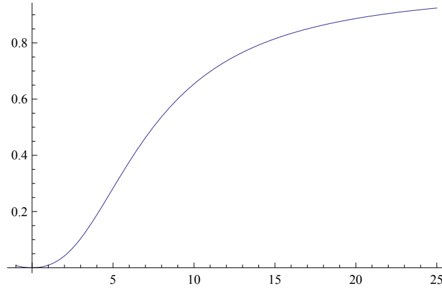
Figure 1.1: The normalized pair correlation function k^\perp(\lambda) in the normal direction u^\perp for the sphere in \mathbb{C}^2
